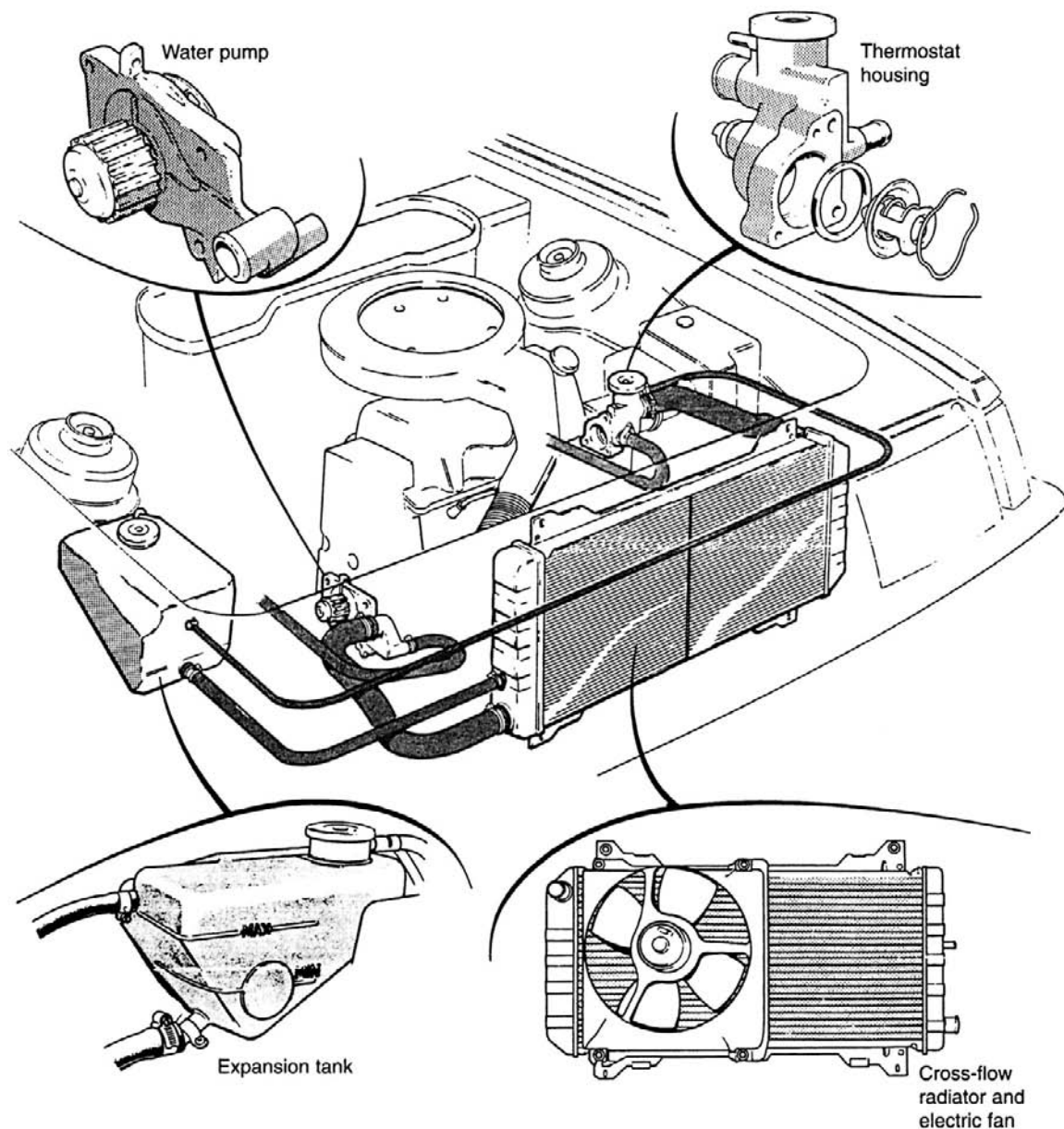
Fig. 13.20 Layout for the Ford transverse engine
