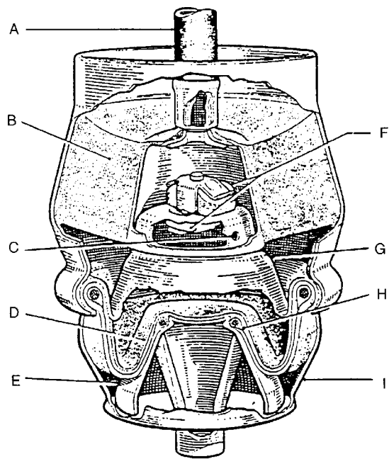
A – Fluid outlet to rear unit F – Damper valves B – Rubber spring G – Dividing member C – Fluid bleed hole H – Reinforcing in diaphragm D – Rubber diaphragm I – Tapered outer cylinder E – Tapered piston
