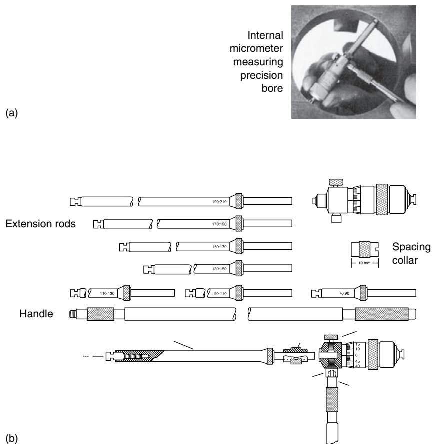
Fig. 31.9 An internal micrometer. (Reproduced with the kind permission of Bowers Metrology Group.)
