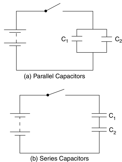
Fig. 25.34 Capacitors in parallel and in series
