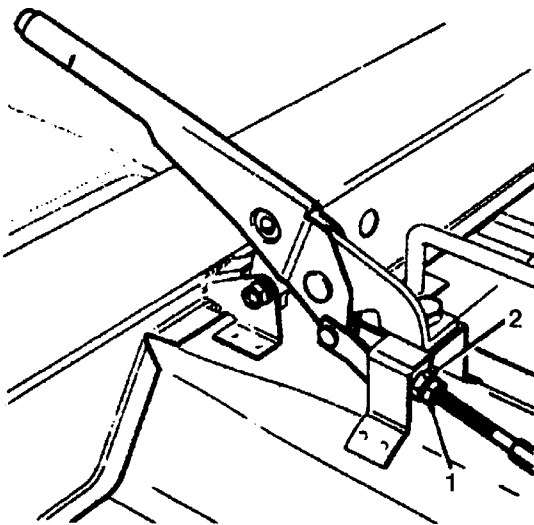
Fig. 21.8 Handbrake cable adjustment
