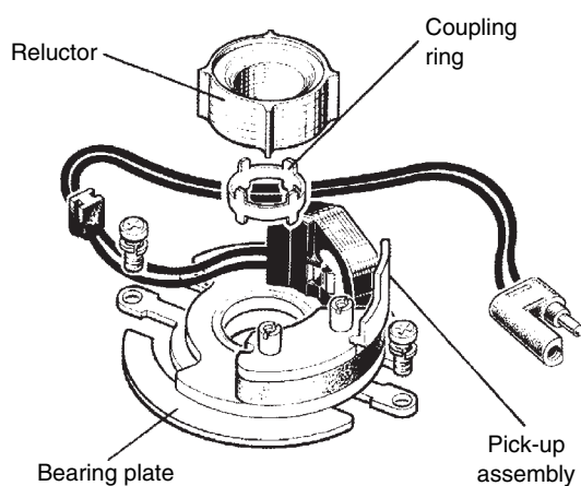
Fig. 27.9 Reluctor and pick-up assembly
