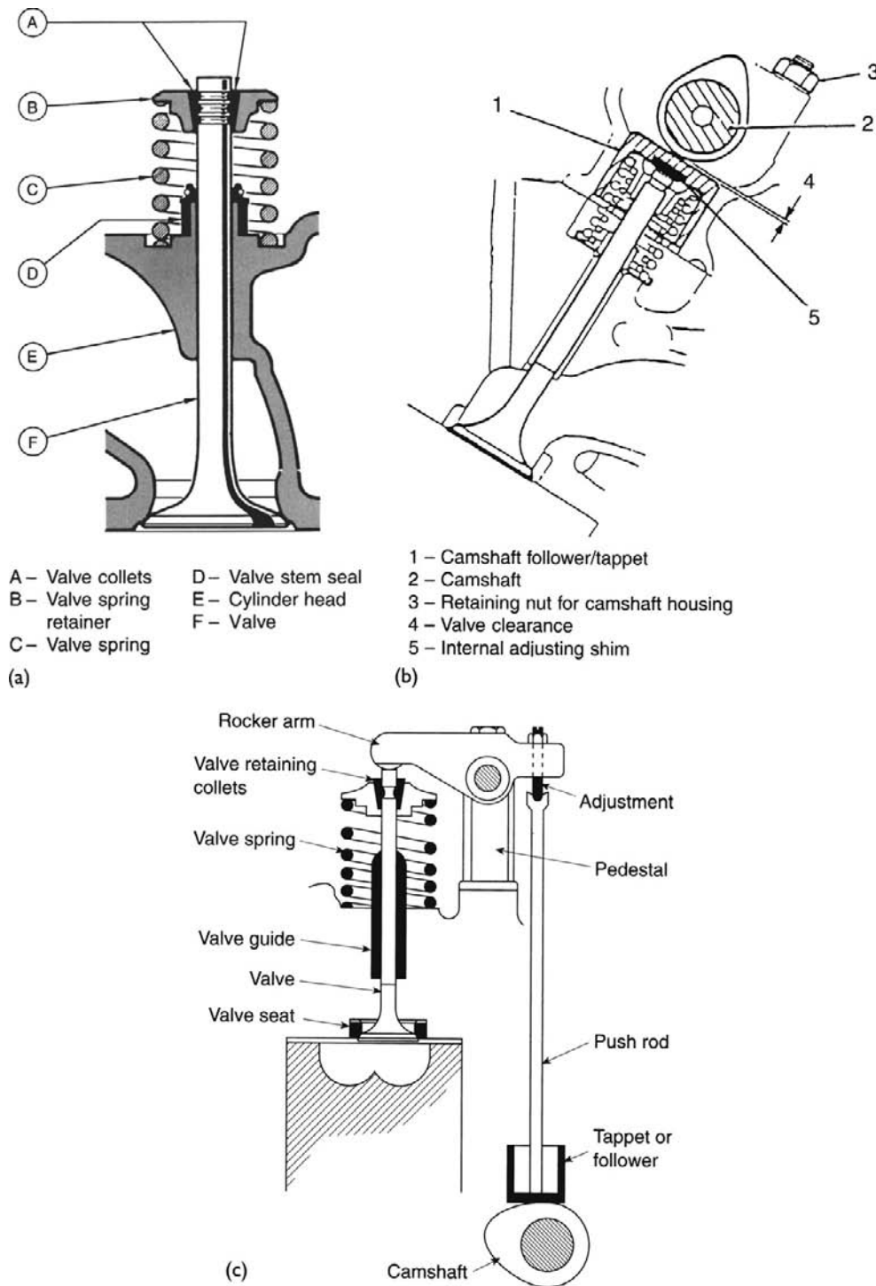
Fig. 3.1 Valve details
