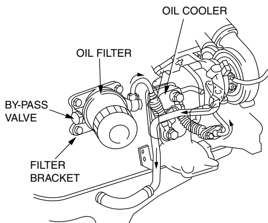
Fig. 12.30 An oil-to-water cooler
