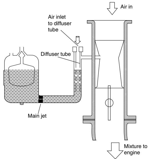
Fig. 9.3 Diffuser tube air bleed compensation
