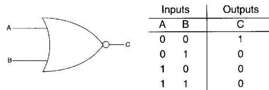
Fig. 25.51 NOR gate and truth table
